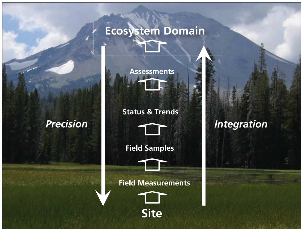
Figure 4.7. Relationship between measurement precision and integration for Klamath Network vital signs monitoring.
