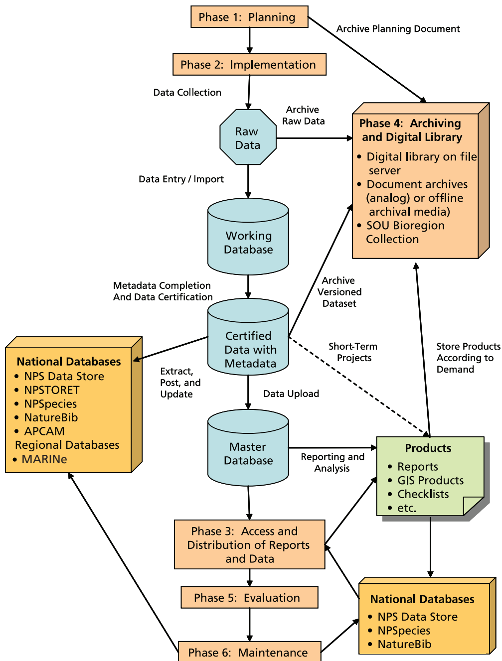
Figure 6.2. Diagram of the data life cycle, illustrating the major data management activities during the life of a project.
