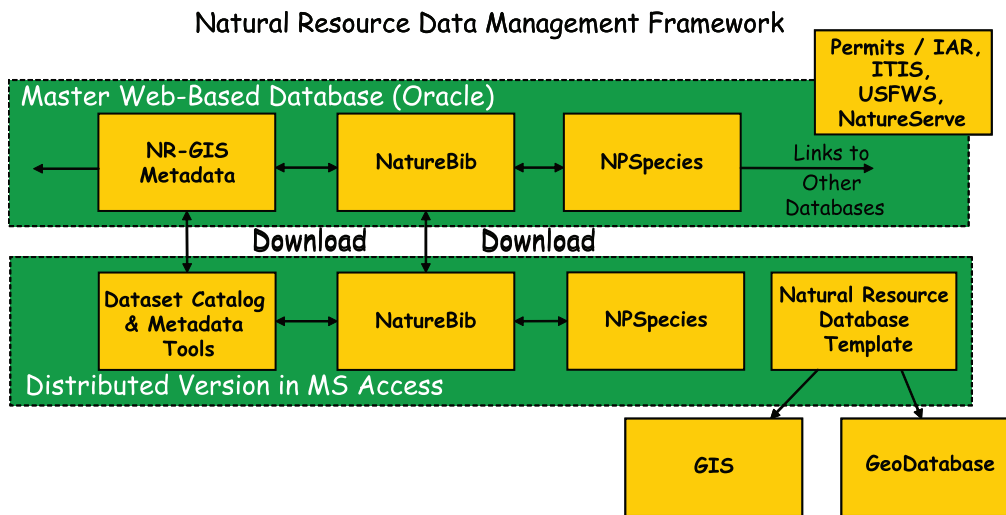
Figure 6.1. Model of the national-level application architecture for integrated natural resources databases.
